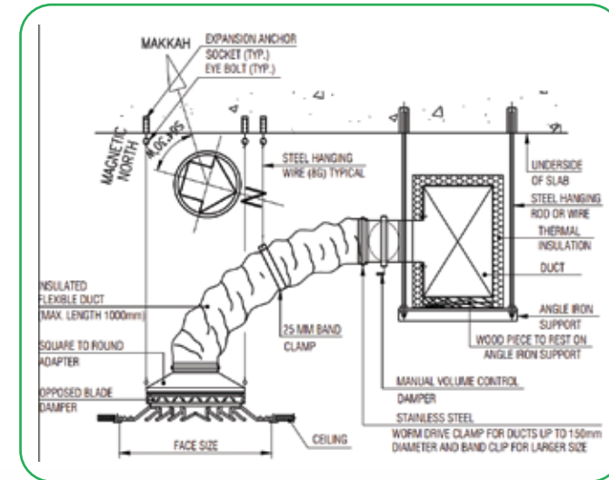
DIFFUSER INSTALLATION DETAIL
